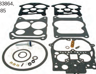
Rochester 4 Barrel (1977-1989)
